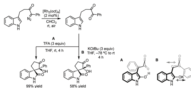
Scheme 34 Taylor and Unsworth's approach using indole nucleophilicity.
