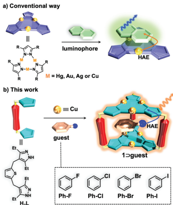
Scheme 1 Conceptual representation of (a) triggering the phosphorescence of organic arenes utilizing the external HAEs of CTCs and (b) enhancing the phosphorescence of \text{Cu}_6\text{L}_3 cage 1 by the encapsulation of halogen aromatic guests.
