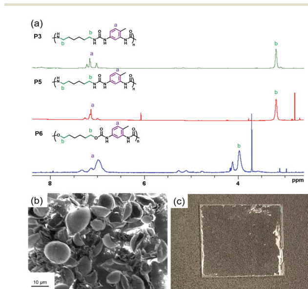
Fig. 3 (a) ^1\text{H} -NMR spectra of polyurea/urethane nanocapsules (entries P3, 5 and 6) in acetone- d_6 : TFA (40 : 60). (b) SEM micrograph of polyurea microcapsules prepared by interfacial polymerization in an oil-in-water emulsion. (c) Photograph of a polyurethane coating prepared by the reaction between resorcinol and HMDI.
