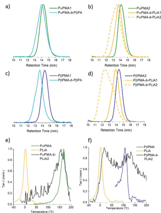
Fig. 1 (a–d) GPC traces showing controlled chain extension of P \alpha PMA with (a) \beta PA and (b) LiA, and of P \beta PMA with (c) \beta PA and (d) LiA. (e and f) DMA traces for (e) P \alpha PMA- b -PLiA2 and (f) P \beta PMA- b -PLiA2, overlaid with the DMA traces of the relevant homopolymers (synthesised to full conversion).
