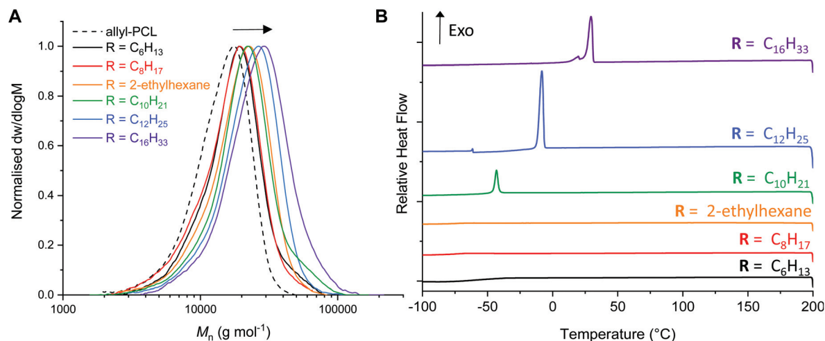
Fig. 3 (a) Poly(ε-allyl-ε-caprolactone) functionalised with various thiols: 1-hexanethiol, 1-octanethiol, 2-ethyl hexanethiol, 1-decanethiol, 1-dodecanethiol and 1-hexadecanethiol, compared to poly(ε-allyl-ε-caprolactone). Size exclusion chromatogram with molecular weights determined against poly(styrene) standards using CHCl 3 (0.5% NEt 3 ) as eluent. (b) Differential scanning calorimetry (DSC) for 2 nd cooling cycle (200 to −100 °C, 10 °C min −1 ) showing crystallisation of the polymer.
