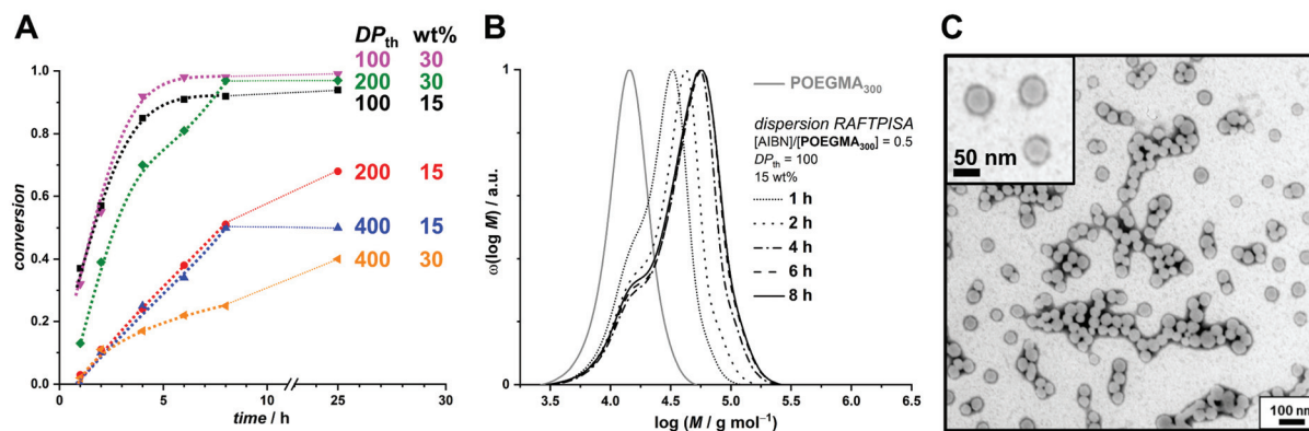
Fig. 3 (A) Conversion vs. time plots for PBBMA dispersion RAFTPISA with POEGMA 300 at [AIBN]/[POEGMA_{300}] = 0.5 at various solids contents and DP_{th} . (B) Size-exclusion chromatograms of polymers obtained by PBBMA dispersion RAFTPISA in methanol at 70 °C with POEGMA 300 at [AIBN]/[POEGMA_{300}] = 0.5 , DP_{th} = 100 , and 15 wt% solids content (entry 7, Table S3†). (C) Transmission electron micrograph of nanoparticles obtained after 25 h under conditions corresponding to B (entry 7, Table S3†).
