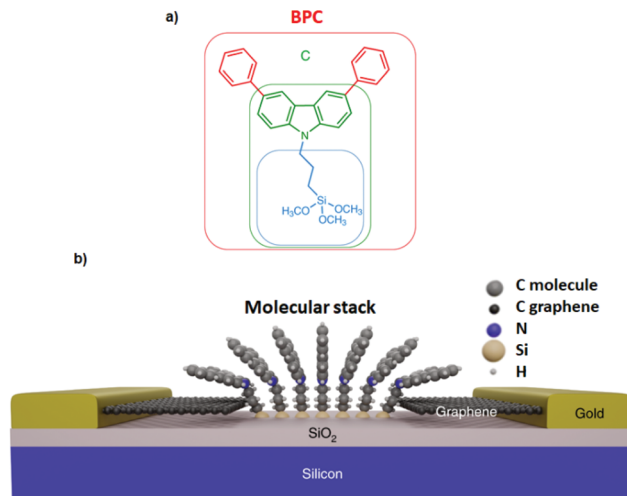
Fig. 2 (a) Molecular structure. (b) Schematic of the molecular junction including molecules bridged via different \pi – \pi -stacking into graphene. Reprinted with permission from El Abbassi et al. , Nat. Nanotechnol. , 2019, 14 , 957. Copyright 2019 Nature Publishing Group.
