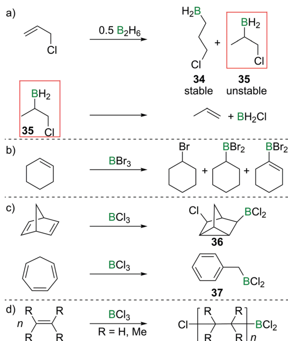
Scheme 16 (a) Hydroboration of allyl chloride gives 3-chloropropylborane (34) and 1-chloro-2-propylborane (35); the latter decomposes upon elimination of BH_2Cl to give propene. (b) Reaction of cyclohexene with BBr_3 yields a mixture of products. (c) and (d) Select examples of BCl_3 initiated cationic rearrangements or polymerisation of alkenes.
