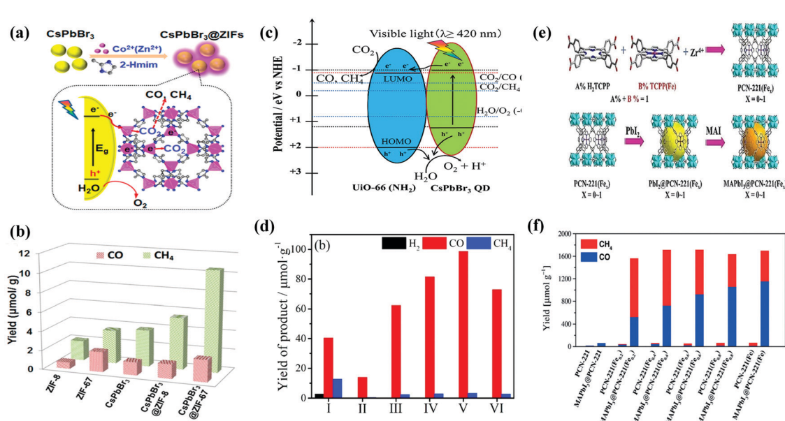
Fig. 13 (a) Schematic illustration of the fabrication process and CO 2 photoreduction process of CsPbBr 3 /ZIFs. (b) The product yield after 3 h of photocatalytic reaction. (a and b) Reprinted with permission from ref. 102, Copyright 2018 American Chemical Society. (c) Schematic illustration of a possible mechanism of photocatalytic CO 2 reduction. (d) Photocatalytic CO 2 reduction performance for CsPbBr 3 QDs and x%-CsPbBr 3 QDs/UiO-66(NH 2 ) nanocomposite. (c and d) Reprinted from ref. 113, Copyright (2019), with permission from Elsevier. (e) Schematic representation for the synthesis of PCN-221(Fe x ) MOF and MAPbI 3 @PCN221(Fe x ) composite photocatalysts for stable and product selective CO 2 reduction. (f) Histogram of product formation using PCN-221(Fe x ) and MAPbI 3 @PCN-221(Fe x ). (e and f) Reproduced with permission from ref. 45, Copyright 2019 Wiley.
