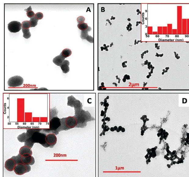
Fig. 5 TEM images of SnO 2 NPs at different magnification, synthesized via electron beam irradiation. (A) 35 kGy, (B) 72 kGy, (C) 107 kGy and (D) 143 kGy in the reline matrix.
