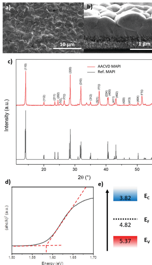
Fig. 1 (a) Topographical SEM image of MAPI film deposited via AACVD showing large grains. (b) Cross-section SEM image of deposited film, with layers of FTO and mesoporous \text{TiO}_2 visible. (c) XRD patterns of films deposited via AACVD and MAPI reference pattern (ICSD 250735). 31 (d) Tauc plot of AACVD MAPI derived from absorption data. (e) Band diagram of AACVD perovskite material, determined by a combination of UV-Vis, ambient photoemission spectroscopy and Kelvin Probe measurements.
