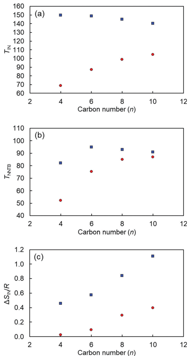
Fig. 3 (a) T_{IN} , (b) T_{NTB} , and (c) \Delta S_{IN}/R values as a function of n for CBCOOnSCB with n = 4, 6, 8 , and 10 (red circles) and CBOCOnSCB with n = 4, 6, 8 , and 10 (blue squares).
