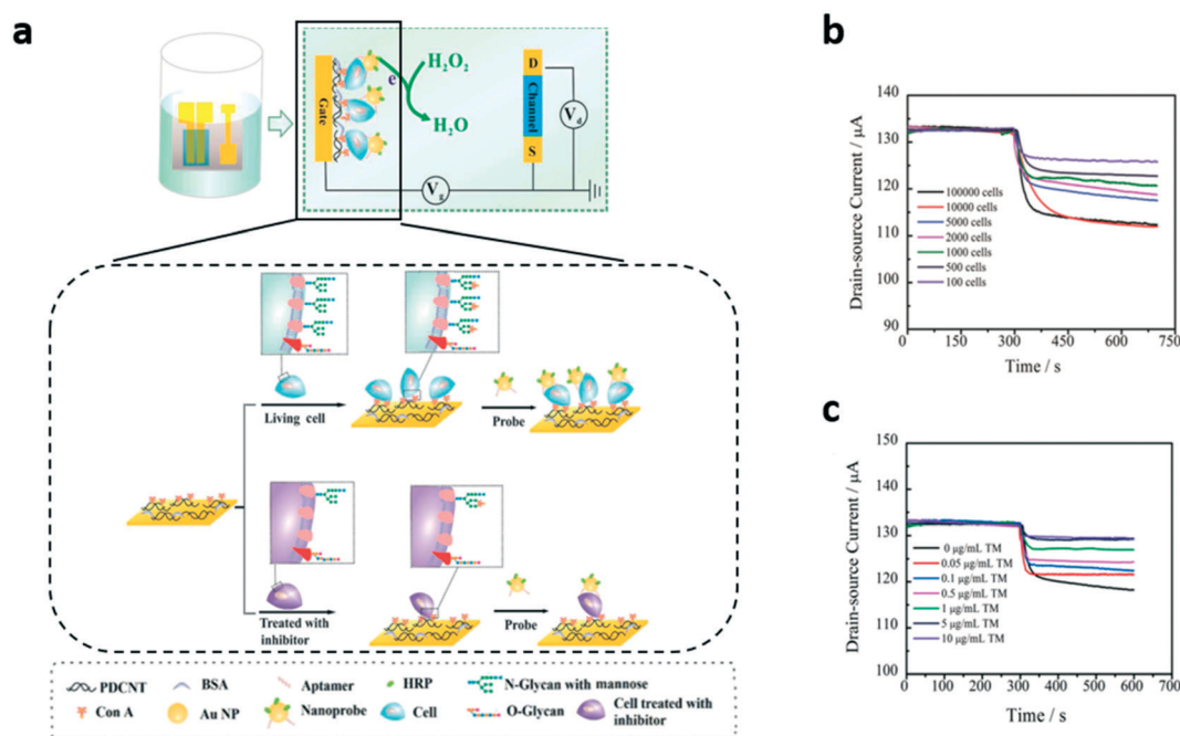
Fig. 7 Planar OEET for in vitro monitoring of non-electrogenic cells. a) Scheme and working principle of the device in ref. 76. The variation of I_D depends on the amount of HRP-functionalized gold nanoparticles (HPR reduces \text{H}_2\text{O}_2 added in solution) captured by the cells adhered onto the gate electrode, and this number depends in turn on the cells' mannose (an N-glycan present on the surface of human breast cancer cells) expression. Thus the I_D increases with the number of living cancer cells plated on the device (b), and decreases with the concentration of an inhibitor of mannose expression with which cells are treated (c). Adapted with permission from ref. 76, Copyright 2018 American Chemical Society.
