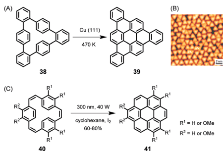
Fig. 6 (A) Cyclodehydrogenation of 38 to tribenzo[a,g,m]coronene 39 . (B) STM image of 39 on Cu(111); V_s = -0.6 V, I = 50 pA, 5 K. 114 Copyright 2010. Adapted with permission from Macmillan Publishers Ltd: Nature Chemistry. (C) Synthesis of coronene compounds via photochemical cyclization of 40 .
