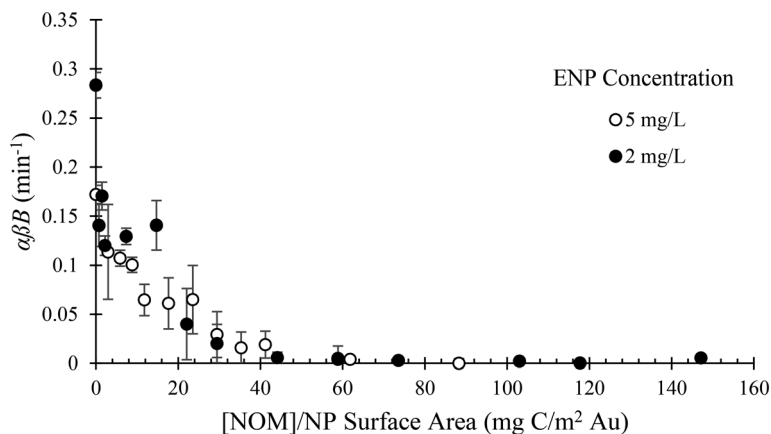
Fig. 4 Pseudo-first order rate constants ( \alpha\beta B ) for attachment of bPEI-AuNPs ( 2\text{ mg L}^{-1} or 5\text{ mg L}^{-1} ) to glass beads ( 20\text{ g L}^{-1} ) in 1\text{ mM} HEPES, 20\text{ mM} NaCl, and varying concentrations of SRNOM. Error bars represent one standard deviation of replicates.
