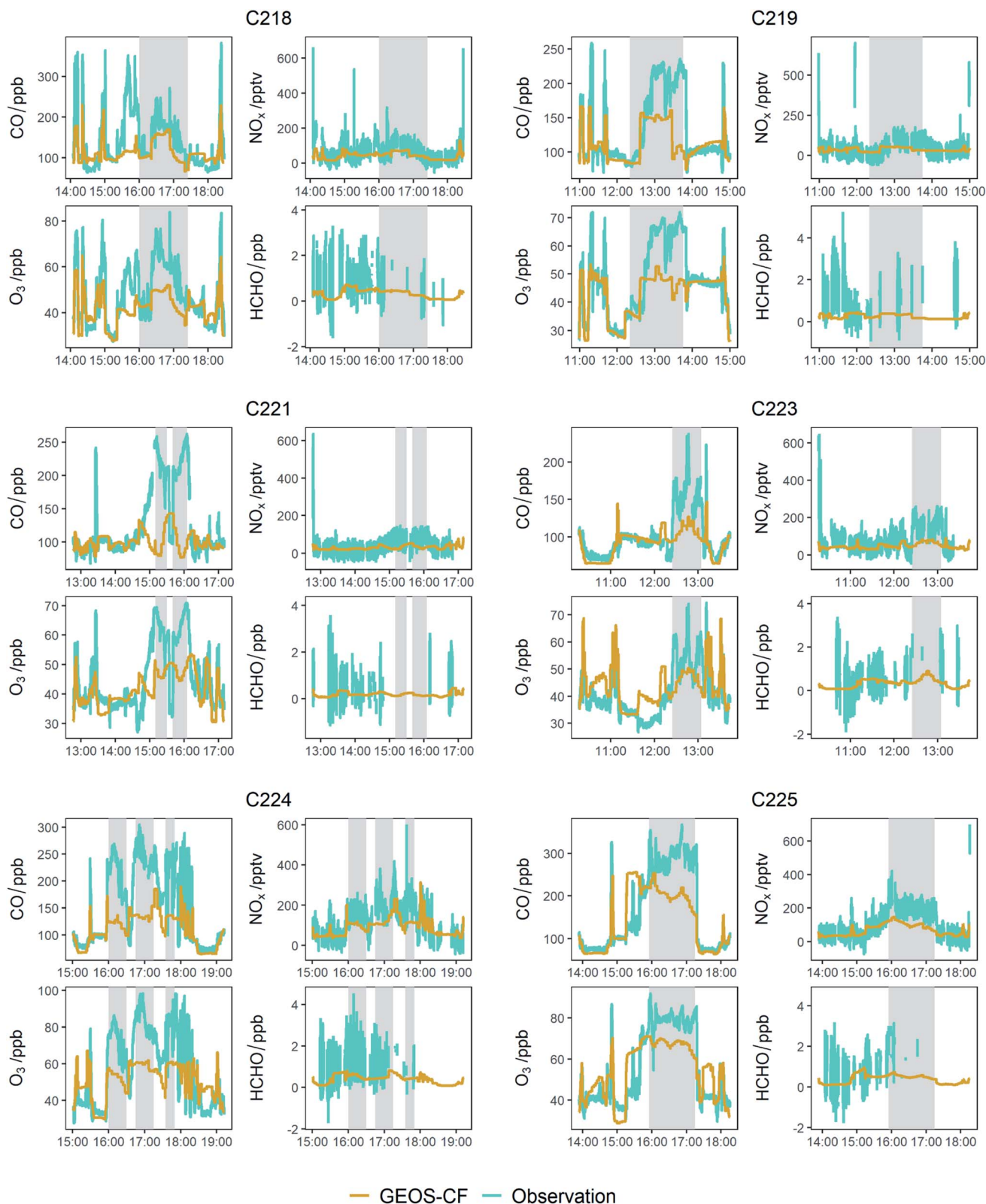
Fig. 8 Time series of measured and modelled (GEOS-CF) \text{O}_3 , \text{CO} , \text{NO}_x and \text{HCHO} .
