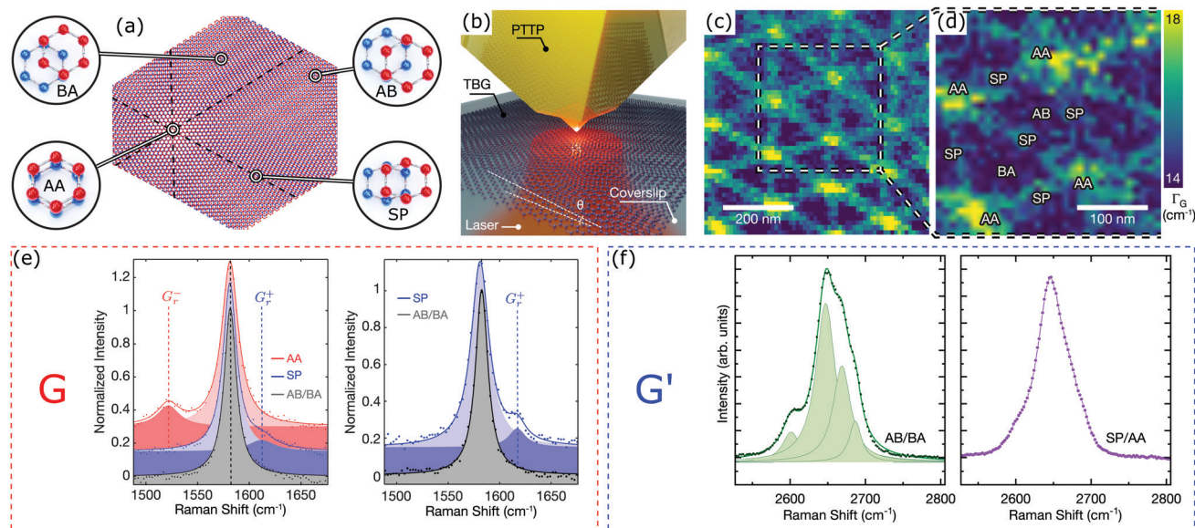
Fig. 6 (a) Representation of rTBG. (b) Sketch of rTBG imaging by nano-Raman highlighting the TERS tip (PTTP – plasmon-tuned-tip pyramid). (c) Nano-Raman TBG map recorded from the G' (also named 2D) band intensity. (d) G-band FWHM nano-Raman map acquired at the dashed square in (c). (e) Nano-Raman G-band spectra recorded in AA (red), SP (blue) and AB/BA regions. The left panel data were acquired in the same sample as in (d), and the right panel data were from another location with a single soliton. (f) Nano-Raman G' spectra from the AB/BA (left) and SP/AA (right) regions. Reproduced with permission from ref. 93.
