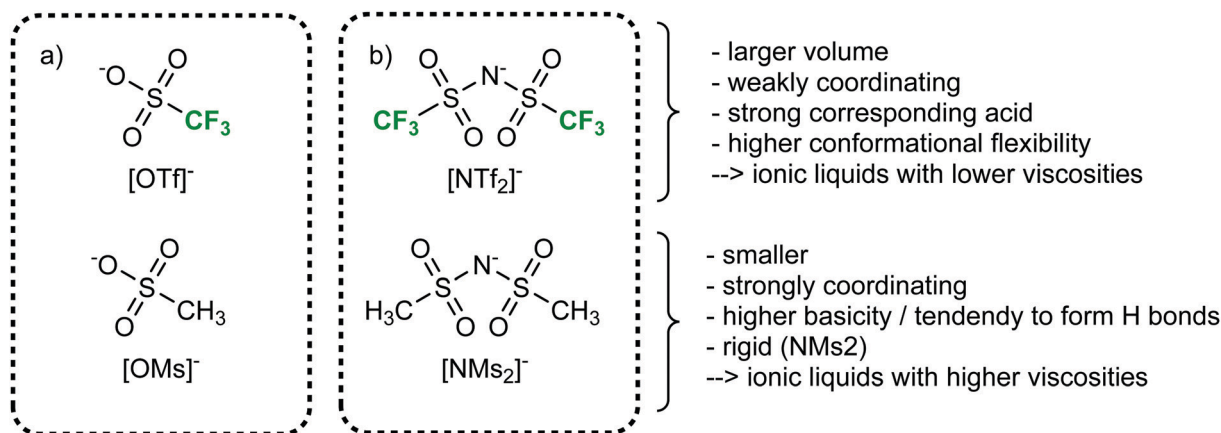
Fig. 24 Fluorinated (top row) and non-fluorinated (bottom row) anions and their typically observed behaviours. Fluorinated anions such as (a) [OTf]^- or [NTf_2]^- are often used for their beneficial physicochemical properties.
