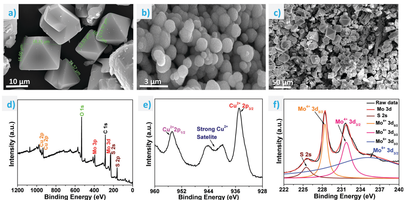
Fig. 2 SEM images of (a) HKUST-1 single crystals, (b) MoS 2 , and (c) HKUST-1 ground sample dropcasted on the MoS 2 support, and the XPS data of the HKUST-1-MoS 2 sample; (d) full XPS spectrum; (e) Cu 2p XPS spectrum; and (f) Mo 3d, S 2s XPS spectrum.
