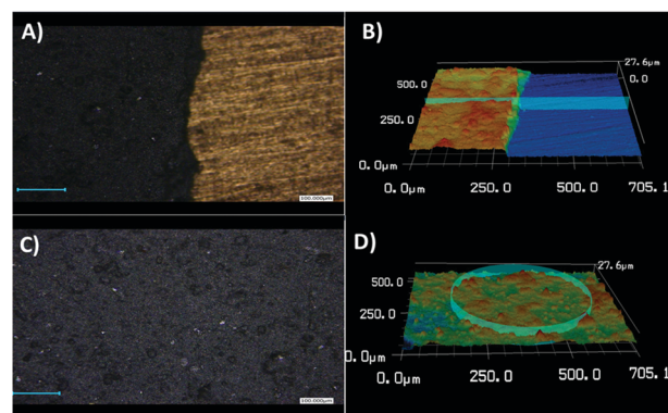
Fig. 2 Height mapping images and 3D views realized with a confocal laser microscope at a magnification of ×50 of WS 2 -COOH film at the cut edge (A and B) with the film on the left and the substrate on the right. Microscope images of the center of the film (C and D).
