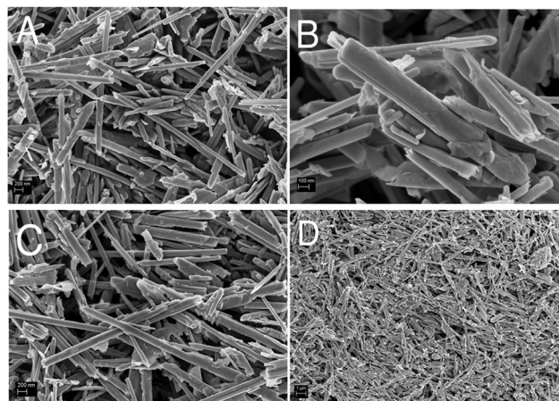
Fig. 1 SEM images of (A and B) as synthesized WS 2 -COOH powder at magnifications of (A) ×20 000 and (B) ×50 000. SEM images of (C and D) thin films of WS 2 -COOH nanotubes at magnifications of (C) ×20 000 and (D) ×5000.
