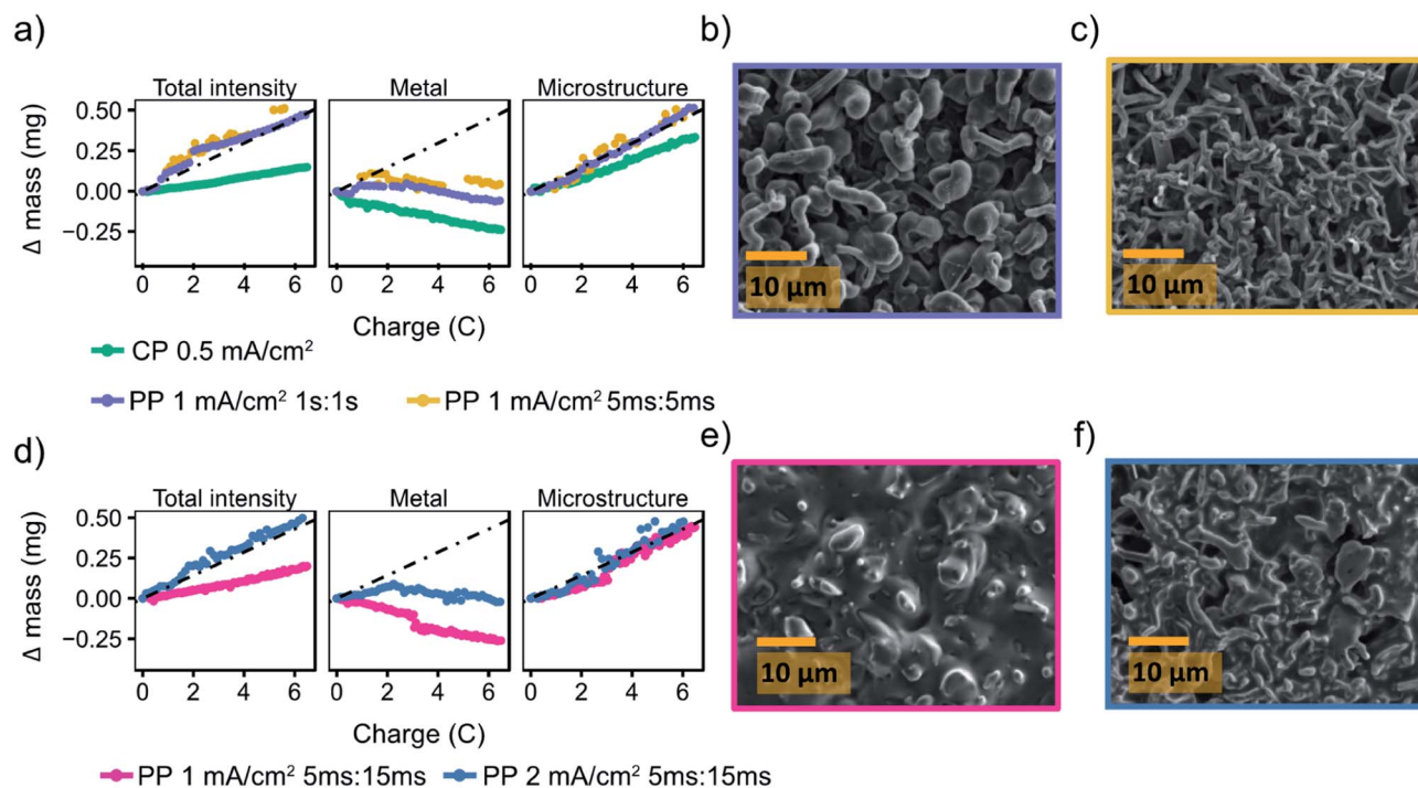
Fig. 6 Pulse plating in LP30 (a) The deconvoluted intensities of the in situ spectra for LP30 during constant plating (CP) at 0.5 mA cm -2 (green, also plotted in Fig. 2) and pulse plating (PP) at 1 mA cm -2 with T_{\text{ON}}, T_{\text{OFF}} = 1 s (purple) and T_{\text{ON}}, T_{\text{OFF}} = 5 ms (yellow). The dashed line indicates m_{\text{echem}} , the mass deposited according to the current passed by the electrochemistry. SEM images of the Li metal morphology using 1 mA cm -2 and (b) T_{\text{ON}}, T_{\text{OFF}} = 1 s (c) T_{\text{ON}}, T_{\text{OFF}} = 5 ms. (d) The deconvoluted intensities of the in situ spectra during pulse plating with T_{\text{ON}} : T_{\text{OFF}} = 5 ms : 15 ms using current densities of 1 mA cm -2 (pink) and 2 mA cm -2 (blue). SEM images of the Li metal morphology using T_{\text{ON}} : T_{\text{OFF}} = 5 ms : 15 ms and (e) 1 mA cm -2 (f) 2 mA cm -2 .
