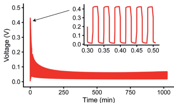
Fig. 5 Representative pulsed current plot for a symmetric Li in situ cell at 1 mA cm -2 with T_{\text{ON}}, T_{\text{OFF}} = 1 s in the LP30 + FEC electrolyte, also shown in Fig. S26.†
