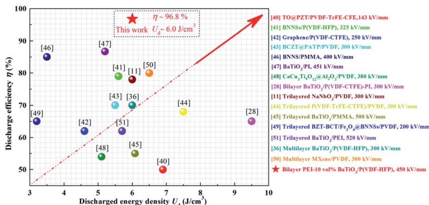
Fig. 6 Comparison of energy density and efficiency of this work (PEI-10 vol% \text{BaTiO}_3/\text{P(VDF-HFP)} composite) and reported results.
