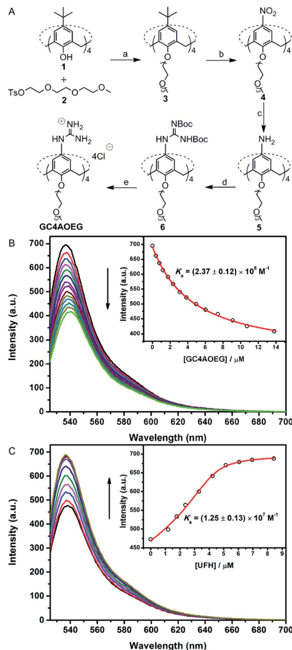
Fig. 2 Synthetic route of GC4AOEG and fluorescence titrations. (A) NaH, dry DMF, and 75 °C; (b) HNO 3 , AcOH, dry CH 2 Cl 2 , and r.t.; (c) SnCl 2 ·2H 2 O, C 2 H 5 OH/AcOEt (1 : 1, v/v), and reflux; (d) 1,3-bis(tert-butoxycarbonyl)-2-methyl-2-thiopseudourea, Et 3 N, AgNO 3 , dry CH 2 Cl 2 , and r.t.; (e) SnCl 4 , AcOEt, and r.t. (B) Direct fluorescence titration of 0.5 μM EY with different concentrations of GC4AOEG (up to 13.8 μM) in HEPES buffer (10 mM, pH = 7.4), and λ ex = 517 nm. (Inset) The associated titration curve at λ em = 537 nm and best fit according to a 1 : 1 binding stoichiometry. (C) Competitive fluorescence titration of GC4AOEG-EY (4.0/0.5 μM) with UFH (up to 8.4 μM in the concentration of monomer units of UFH), and λ ex = 517 nm. (Inset) The associated titration curve at λ em = 537 nm and best fit according to a n : 1 competitive binding model, where n = 0.88.
