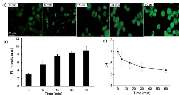
Fig. 5 (a) Real time fluorescence imaging of A549 cells stained with the probe PS-OH (20 \mu\text{M} ) up to 60 minutes after treatment with 500 \mu\text{M} H 2 O 2 . (b) A plot of the fluorescence intensity with time during apoptosis. (c) Quantification of the corresponding dynamic changes in pH at different time points in comparison with the calibration curve in Fig. 3c.
