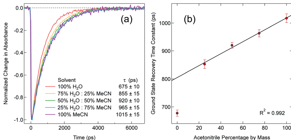
Fig. 8 (a) Time-resolved absorption data for ground-state recovery of [\text{Fe}(\text{bpy})_3]\text{Br}_2 in binary solvent mixtures of water ( \text{H}_2\text{O} ) and acetonitrile ( \text{MeCN} ) following ^1\text{A}_1 \rightarrow ^1\text{MLCT} excitation at 550 nm. (b) Fit of the time constants obtained from the data in part (a), showing a linear correlation between the kinetics of ground state recovery and the mass percentage of acetonitrile in the solvent mixture. The data point for pure water ( i.e. , 0% acetonitrile) was not included in the fit.
