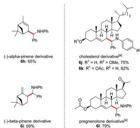
Fig. 1 Late-stage diversification of complex molecules. Reaction conditions: imine 1 (0.2 mmol), alkene 2 (1.0 mmol), \text{Li}_2\text{CO}_3 (20 mol%), i\text{Pr}_3\text{SiSH} 4 (5 mol%), 3a (1 mol%), DMF (1.0 mL), 24 W LEDs (450 nm), rt, 24 h, for dr see ESI† a 2 (0.6 mmol), i\text{Pr}_3\text{SiSH} 4 (10 mol%), DMF (2 mL). b Isomers ratios: 6h (1.2 : 1 : 1 : 1), 6i (3 : 3 : 1 : 1), 6j (1.6 : 1.6 : 1 : 1), 6k (1.2 : 1 : 1 : 1), 6l (1.9 : 1.9 : 1).
