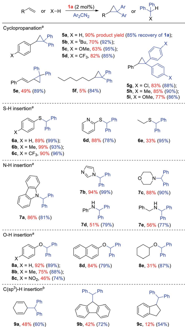
Scheme 4 Intermolecular diarylcarbene transfer reactions catalyzed by 1a . Product yields in red and recovery of 1a (blue) in parentheses. a Conditions: Ph 2 CN 2 (0.2 mmol), substrate (2 mmol), catalyst (0.004 mmol), DCM (1 mL), 40 °C, 12 h, and under Ar. b Conditions: Ph 2 CN 2 (0.2 mmol, added over 3 h), substrate (2 mmol), catalyst (0.004 mmol), DCE (1 mL), 80 °C, 12 h, and under Ar.
