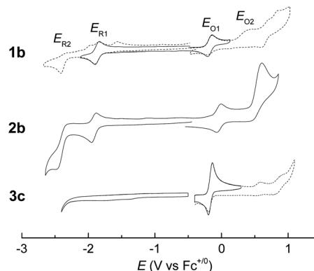
Fig. 7 Cyclic voltammograms of group 8 metal dialkylcarbene complexes supported by the TTP macrocycle, using 0.1 \text{ M } (\text{Bu}_4\text{N})\text{PF}_6 as the electrolyte and at a scan rate of 0.1 \text{ V s}^{-1} . Top: 1b and 2b , measured in DMF with SCE as the reference electrode; E(\text{Fc}^{+/0}) = 0.49 \text{ V} . Bottom: 3c , measured in DCM with \text{Ag}/\text{AgCl} as the reference electrode; E(\text{Fc}^{+/0}) = 0.40 \text{ V} . Dotted lines indicate irreversible redox events.
