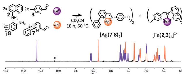
Fig. 6 Top – Generation of complexes [\text{Ag}(\mathbf{7},\mathbf{8})_2]^+ and [\text{Fe}(\mathbf{2},\mathbf{3})_2]^{2+} through the self-sorting of their initial reactants. Reaction conditions: 2 : 3 : 7 : 8 : \text{Ag}(\text{BF}_4) : \text{Fe}(\text{BF}_4)_2 (2 : 2 : 2 : 2 : 1 : 1), \text{CD}_3\text{CN} , 60 °C, 18 h. Bottom – Partial ^1\text{H} NMR spectrum (400 MHz, \text{CD}_3\text{CN} , 297 K) of the crude reaction mixture after 18 h at 60 °C. The diagnostic signals of the complexes are colour coded, [\text{Ag}(\mathbf{7},\mathbf{8})_2]^+ in orange and [\text{Fe}(\mathbf{2},\mathbf{3})_2]^{2+} in purple; one of the diagnostic signals of the free aldehyde 7 is designated by a grey circle.
