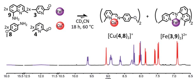
Fig. 5 Top – Generation of complexes [\text{Cu}(\mathbf{4},\mathbf{8})_2]^+ and [\text{Fe}(\mathbf{3},\mathbf{9})_2]^{2+} through the self-sorting of their initial reactants. Reaction conditions: 3 : 4 : 8 : 9 : \text{Cu}(\text{BF}_4) : \text{Fe}(\text{BF}_4)_2 (2 : 2 : 2 : 2 : 1 : 1), \text{CD}_3\text{CN} , 60 °C, 18 h. Bottom – Partial ^1\text{H} NMR spectrum (400 MHz, \text{CD}_3\text{CN} , 297 K) of the crude reaction mixture after 18 h at 60 °C. The diagnostic signals of the complexes are colour coded, [\text{Cu}(\mathbf{4},\mathbf{8})_2]^+ in red and [\text{Fe}(\mathbf{3},\mathbf{9})_2]^{2+} in purple.
