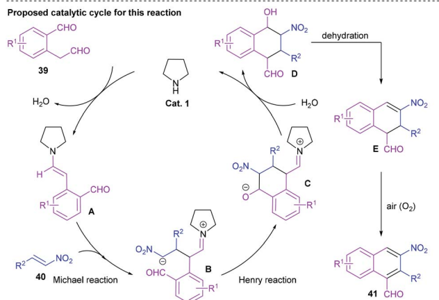
Scheme 11 Pyrrolidine catalyzed [4 + 2] benzannulation to synthesize polysubstituted naphthalene derivatives.
