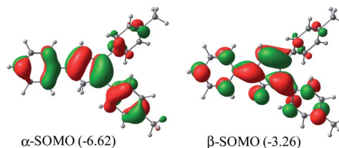
Fig. 6 \alpha - and \beta -SOMO of Me 2 Cp–H ( 1* ) singlet biradical state (in gas phase) calculated at UM062x(GD3)/Def2TZVPP//BP86(GD3)/Def2TZVPP level of theory.
