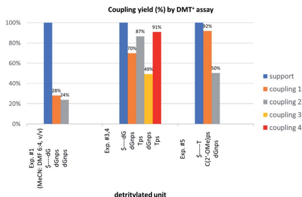
Fig. 3 Coupling yields in the consecutive condensation steps, assessed by \text{DMT}^+ assay at 504 nm. Absorptions of the \text{DMT}^+ cation released from the nucleosides attached to the support (blue bars) are taken as 100%.
