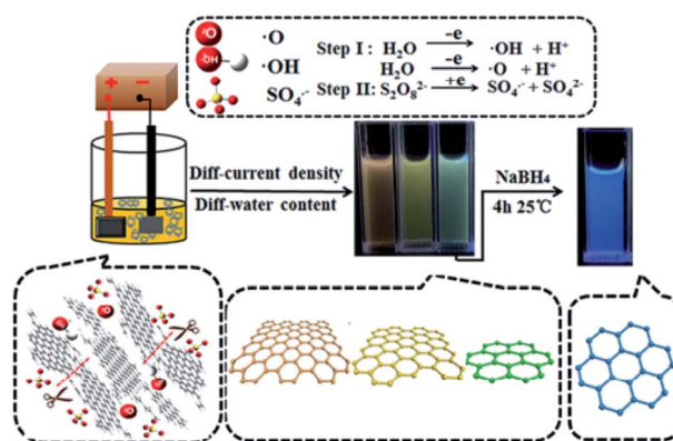
Fig. 1 A schema of the synthetic procedure of multi-color GQDs from the coke. Reprinted with permission. 58 Copyright 2018, Elsevier.
