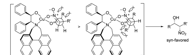
Scheme 15 Asymmetric syn -selective Henry reaction catalyzed by amino alcohol ligand L7.
