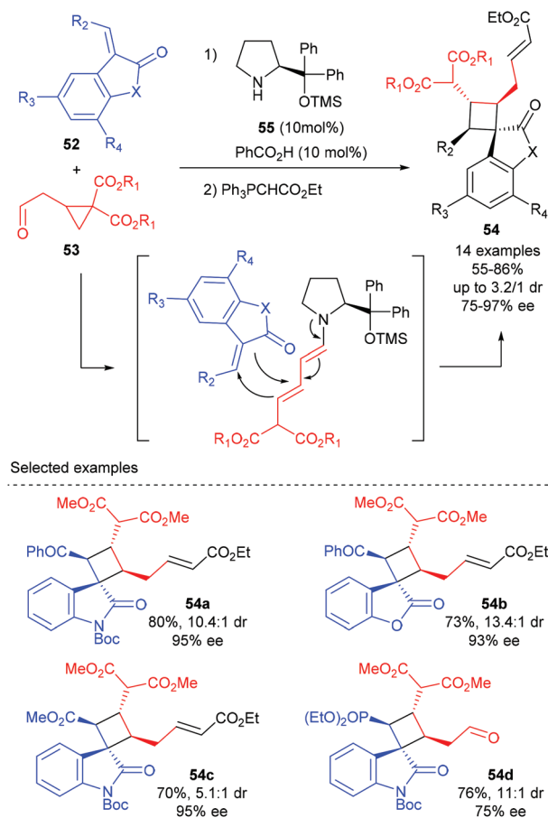
Scheme 15 Enamine-activation of cyclopropanes for highly stereoselective synthesis of cyclobutanes.
