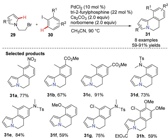
Scheme 4 Palladium-catalyzed alkylation/direct arylation sequence.
