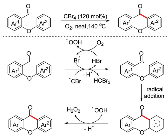
Scheme 69
