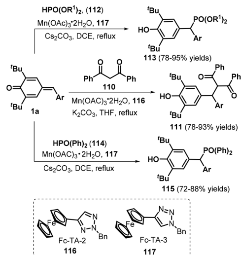
Scheme 23 Manganese-catalyzed 1,6-addition toward functionalized methines.
