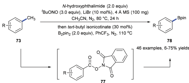
Scheme 17 Sequential radical demethylative \text{C(aryl)-C(CH}_3\text{)} bond cleavage and borylation.
