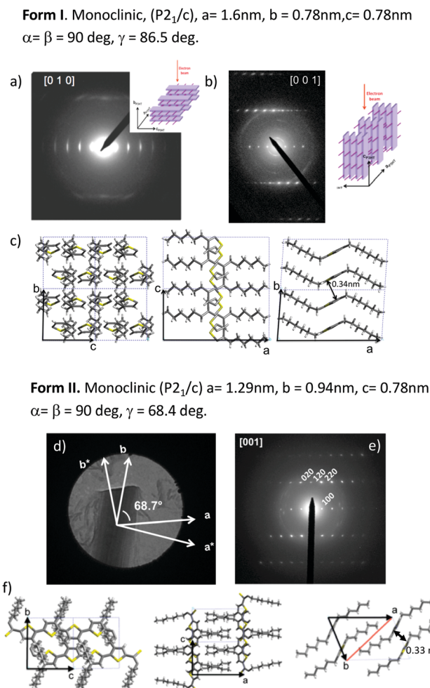
Fig. 4 Comparison of the electron diffraction patterns of P3HT in oriented thin films of form I grown by epitaxy on TCB (a and b) and for a single crystal grown by self-seeding (d and e). In (c) the crystal structure of form I P3HT is illustrated. In (a and b), the orientation of the electron beam with respect to the crystal is highlighted in the insets. In (d), the orientation of the lattice vectors a and c is compared to the direction of the vectors in reciprocal space a* and c* . Reproduced and adapted from ref. 38 (ACS, 2010) and ref. 6 (Wiley-VCH, 2012).
