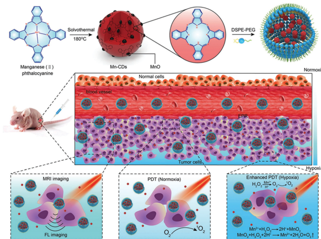
Fig. 12 Schematic illustration of the Mn-CD assembly as an acidic H 2 O 2 -driven oxygen generator to enhance the anticancer efficiency of PDT in a solid tumour. Reprinted with permission from ref. 143. Copyright 2018 John Wiley and Sons.
