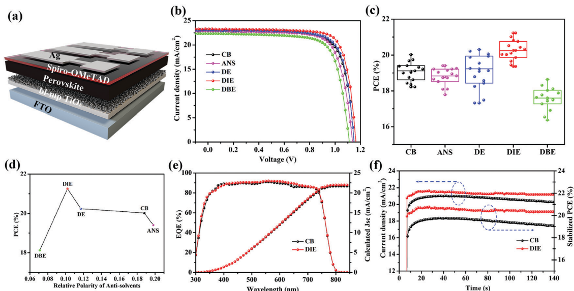
Fig. 3 (a) Schematic representation of the PSC device structure. (b) J - V characteristics of the best \text{Cs}_{0.05}(\text{MA}_{0.17}\text{FA}_{0.83})\text{Pb}(\text{I}_{0.83}\text{Br}_{0.17})_3 perovskite devices and (c) PCE statistics from 15 devices fabricated using CB, ANS, DE, DIE, and DBE as antisolvents, recorded at a scan rate of 20 \text{ mV s}^{-1} . (d) Relationship between the polarity of the antisolvent and the PCE of the PSCs. (e) EQE spectra and integrated current densities of \text{Cs}_{0.05}(\text{MA}_{0.17}\text{FA}_{0.83})\text{Pb}(\text{I}_{0.83}\text{Br}_{0.17})_3 perovskites that had been treated with CB and DIE. (f) Stabilized PCEs of the corresponding triple-mixed PSCs.
