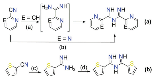
Scheme 4 Synthesis of Py 2 ImAm , Pm 2 ImAm (top) and Th 2 ImAm (bottom). Reagents and conditions: (a) 2-cyanopyridine, acetone, 110 °C; (b) NH 3 , MeCN, RT; (c) (i) NaOMe, MeOH, RT; (ii) NH 4 Cl; (d) NaH, 2-thiophenecarbonitrile, DMSO, RT.
