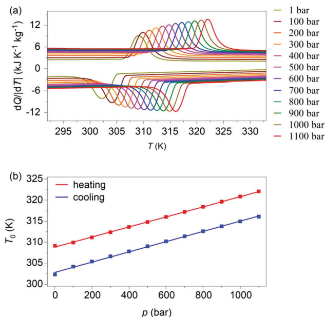
Fig. 2 (a) Heat flow dQ/dT as a function of temperature, at finite applied pressure. (b) Transition temperatures versus pressure, identified using the peak in heat flow dQ/dT .
