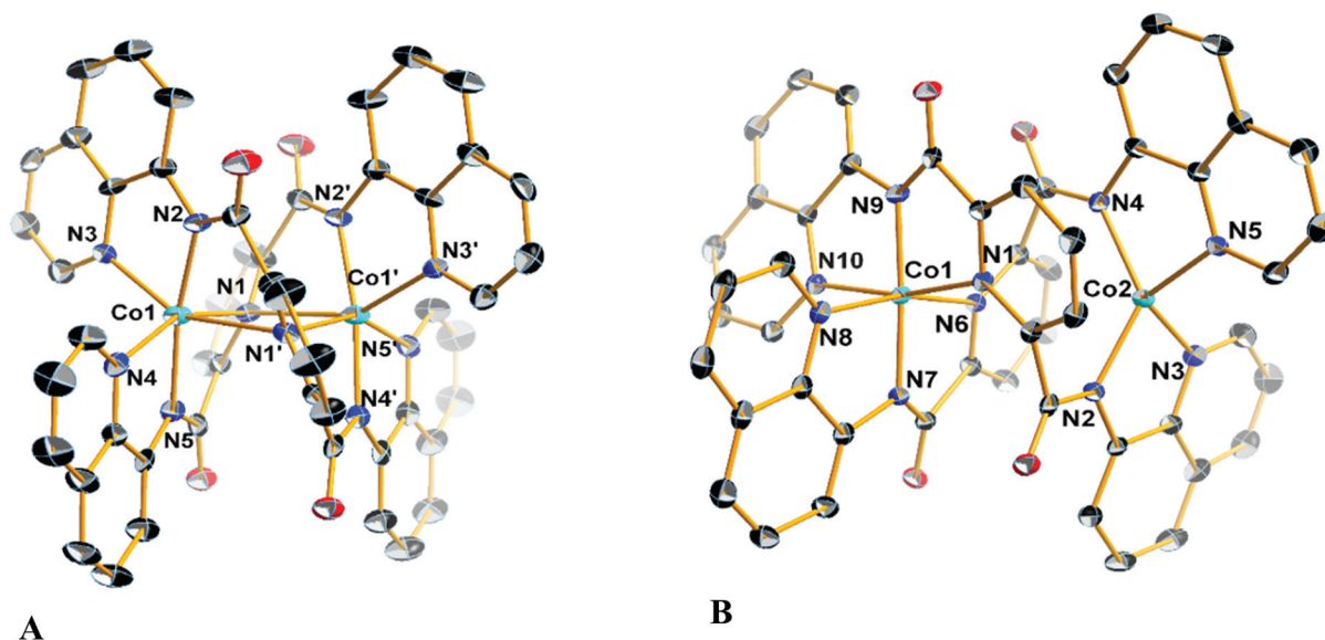
Fig. 1 Molecular structures of (A) the neutral complex in crystals of 1:2CHCl_3 , and (B) cation in crystals of 3:3CH_2Cl_2 with the atom numbering scheme. Displacement ellipsoids are drawn at 50% probability level. Hydrogen atoms have been omitted for clarity. Color code: Co, cyan; C, black; N, blue; O, red.
