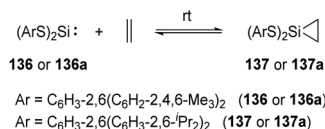
Scheme 55 Reversible addition of ethylene to the acyclic silylenes 136 and 136a .
