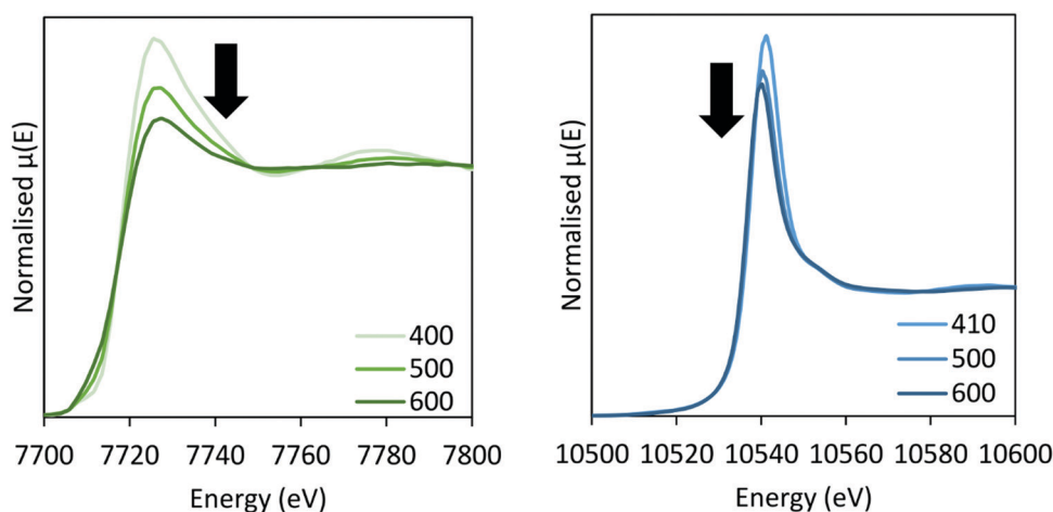
Fig. 11 XANES of the CoRe-gel during ammonia decomposition at the Co K-edge (left) and Re L III -edge (right) between 400–600 °C in 5% NH 3 .
