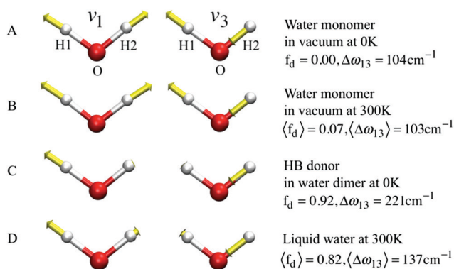
Fig. 11 The symmetric ( \nu_1 ) and asymmetric ( \nu_3 ) stretching modes of a water molecule and their splitting frequency \Delta\omega_{13} = \omega_3 - \omega_1 (A) in vacuum at 0 K, (B) in vacuum at 300 K, (C) of the H-bond donor of a water dimer at 0 K, and (D) in liquid water at 300 K, respectively. See eqn (7) for the definition of f_d . Reprinted with permission from ref. 15. Copyright 2013 American Chemical Society.
