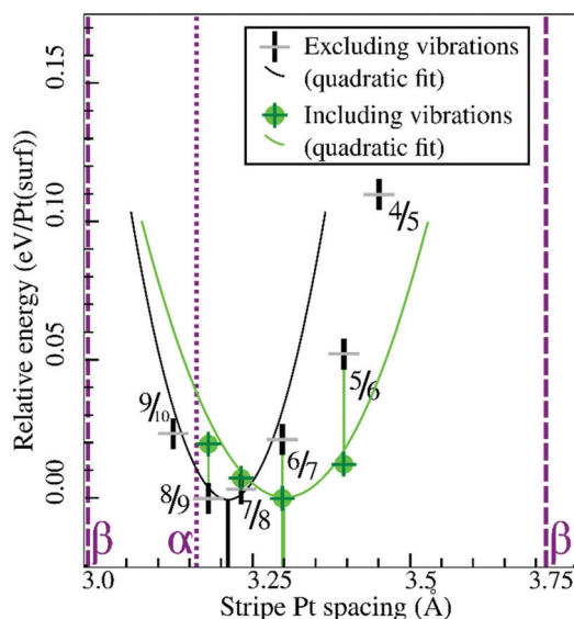
Fig. 7 Comparison of selected stripe energies with and without vibrational energy corrections and their respective quadratic fits; legend in inset.
