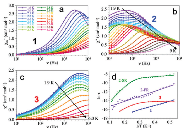
Fig. 3 (a–c) Frequency dependence of \chi_m'' at different temperatures for compounds 1–3 with a DC field of 1000 Oe. Solid lines are the fit to the Debye model with one (for 1 and 3 ) and two (in 2 ) relaxation processes. (d) Arrhenius plot for the relaxation times of compounds 1–3 . Solid lines are the fits to the different models (see text).
