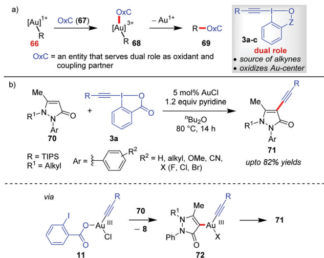
Scheme 14 (a) New coupling partner, 'OxC' for executing Au-catalyzed, redox-neutral C-C cross-coupling; and (b) alkynylation of N-alkyl pyrazolone at the C4-site.
